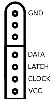
GC Pinout
