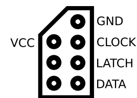
NES Pinout
