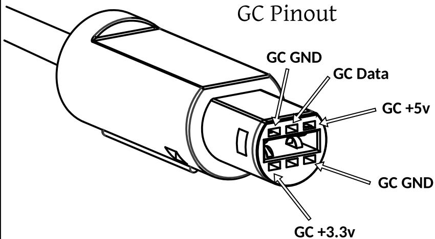
GC Pinout
