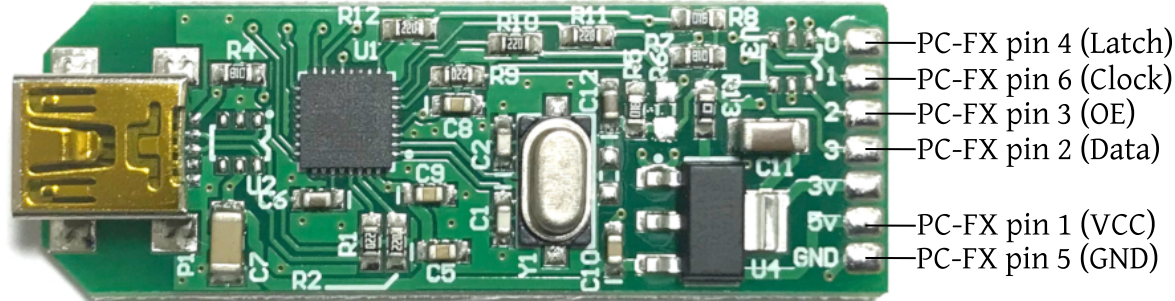
BRD-PCFX-USB
