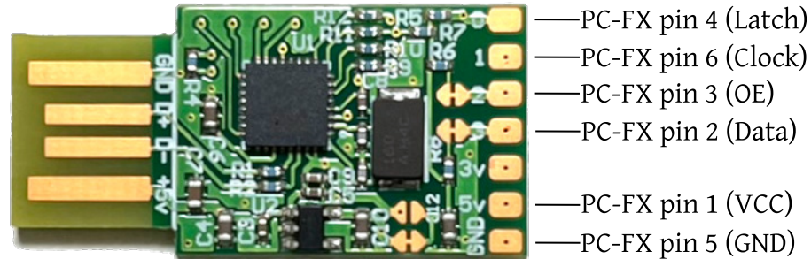
BRD-PCFX-USB-SLD
