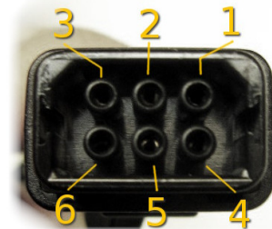
Connector on the controller cable
